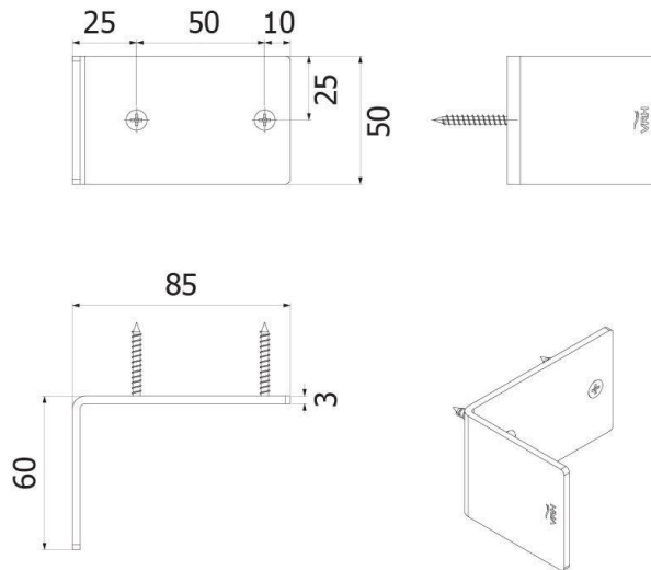
FXVH0-0302AK unit : mm
